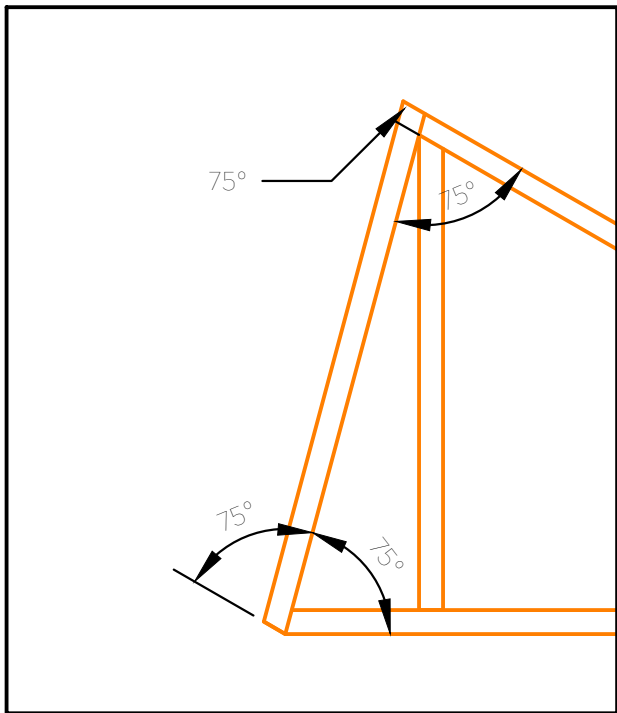
11.4 Platform 2, Section D - Angle Details
