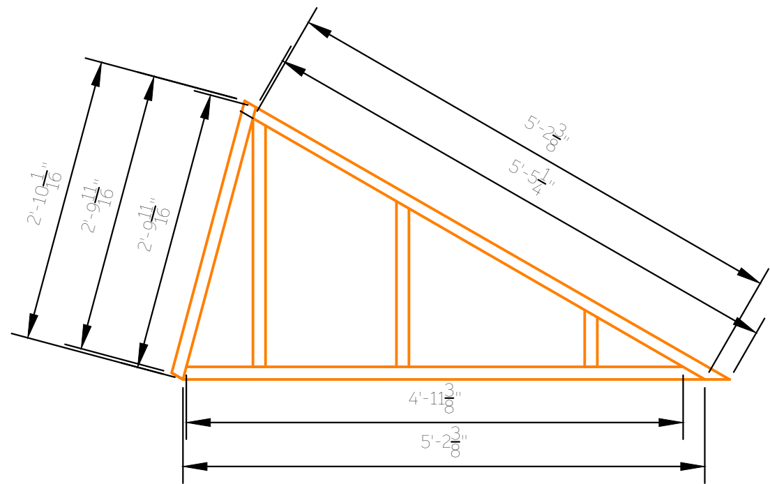
11.3 Platform 2, Section D - Angle Measurements
