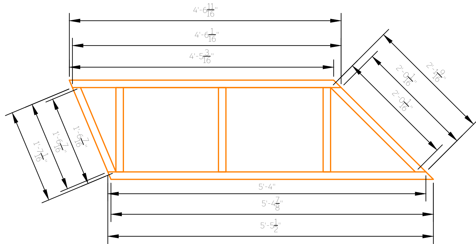
8.3 Platform 2, Section A - Angle Measurements
