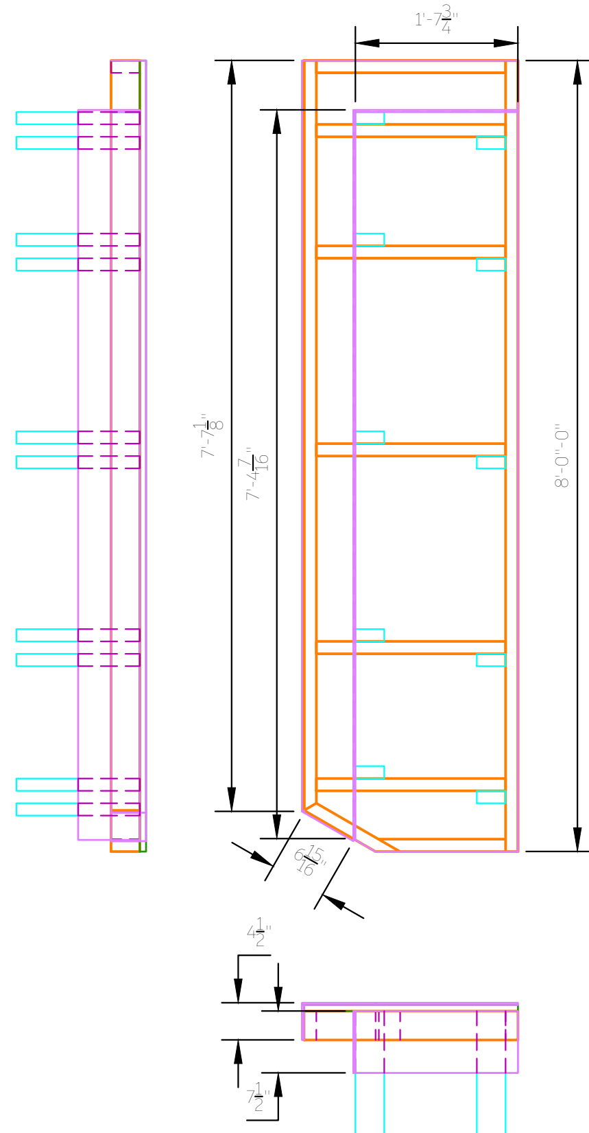
12.5 Platform 2, Section E - MDF Layout TOP, SIDE, FRONT VIEW
