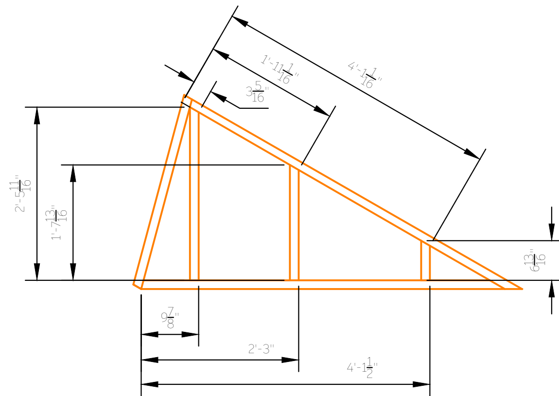
11.1 Platform 2, Section D - Toggle Placement
