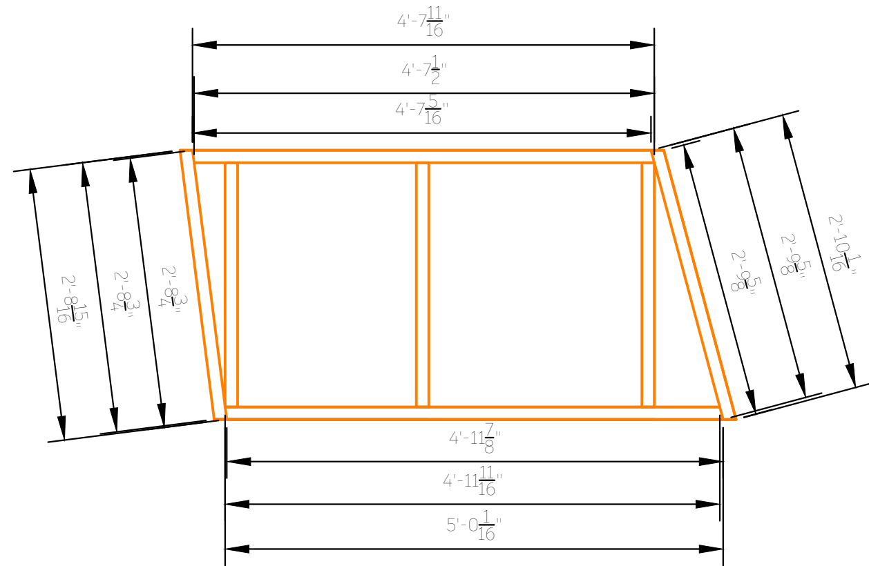
10.3 Platform 2, Section C - Angle Measurements
