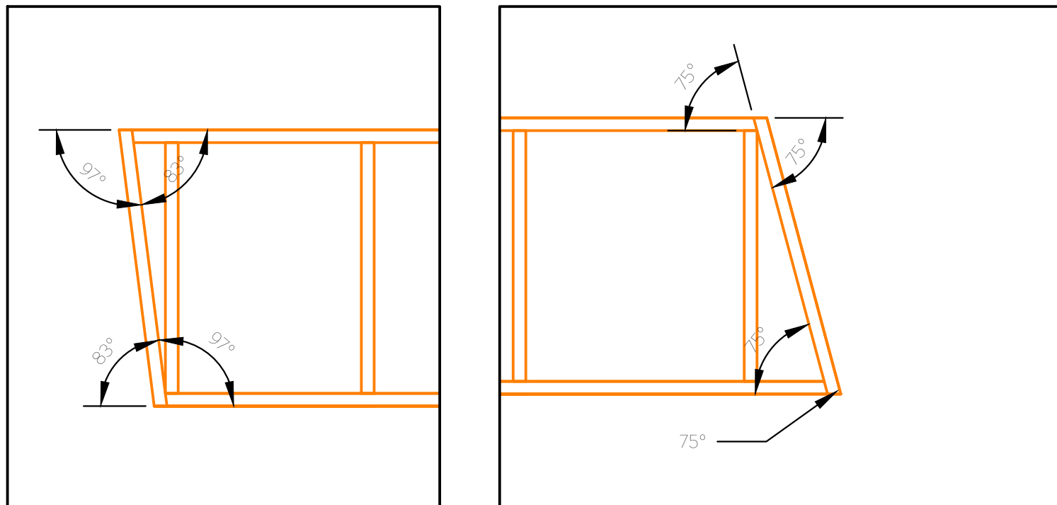
10.4 Platform 2, Section C - Angle Details
