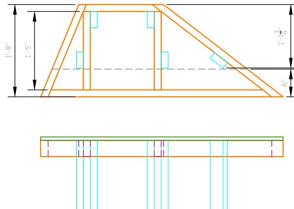
9.2 Platform 2, Section B - Leg Placement/ Inset TOP, SIDE, FRONT VIEW
