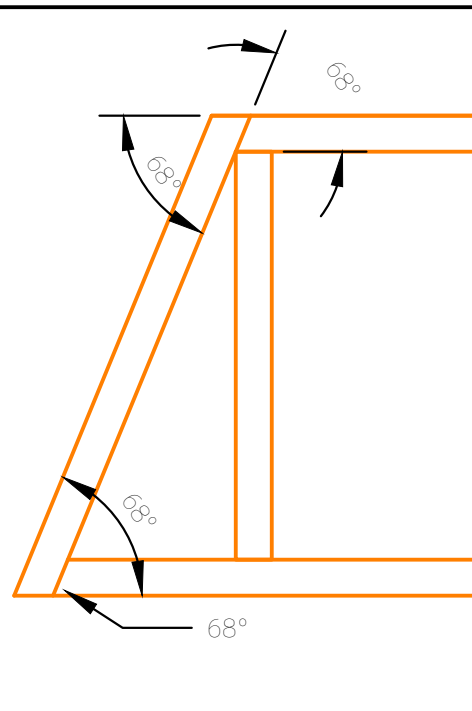
9.4 Platform 2, Section B - Angle Details
