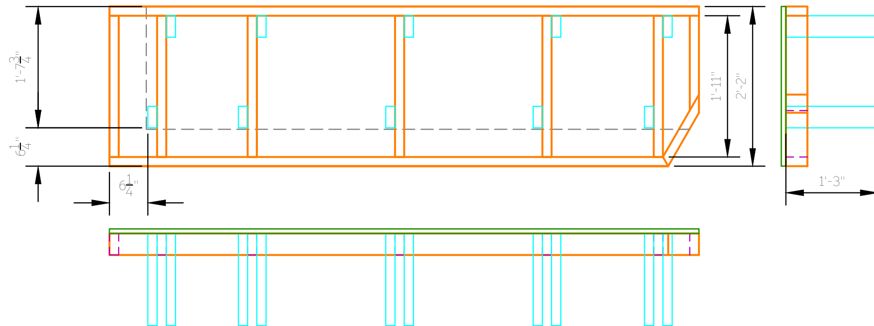
12.2 Platform 2, Section E - Leg Placement/ Inset TOP, SIDE, FRONT VIEW
