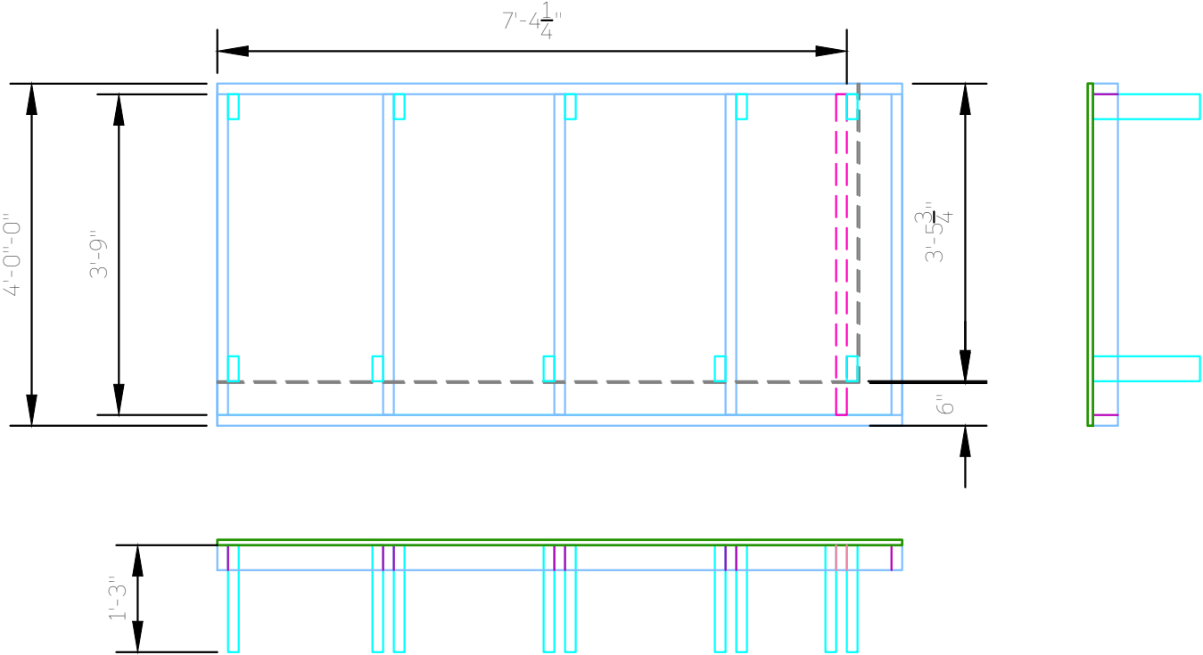
13.1 Platform 2, Section F - Stock Platform Toggle Modifications/ Leg Placement TOP, SIDE, FRONT VIEW
