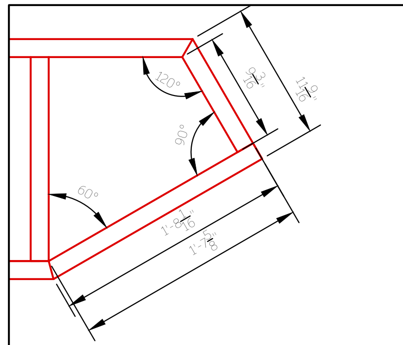
3.3 Platform 1, Section C - Angle Measurements
