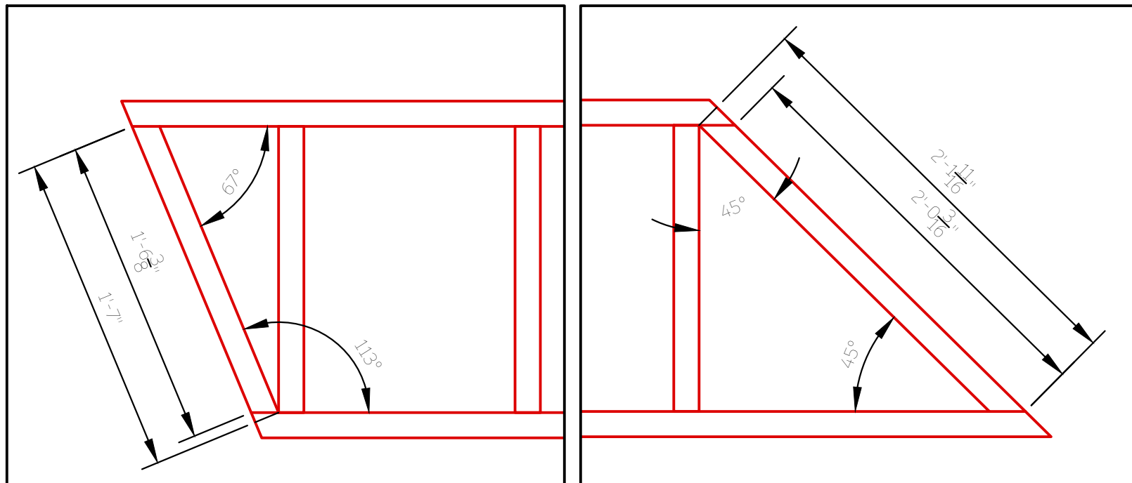
1.4 Platform 1, Section A - Angle Details
