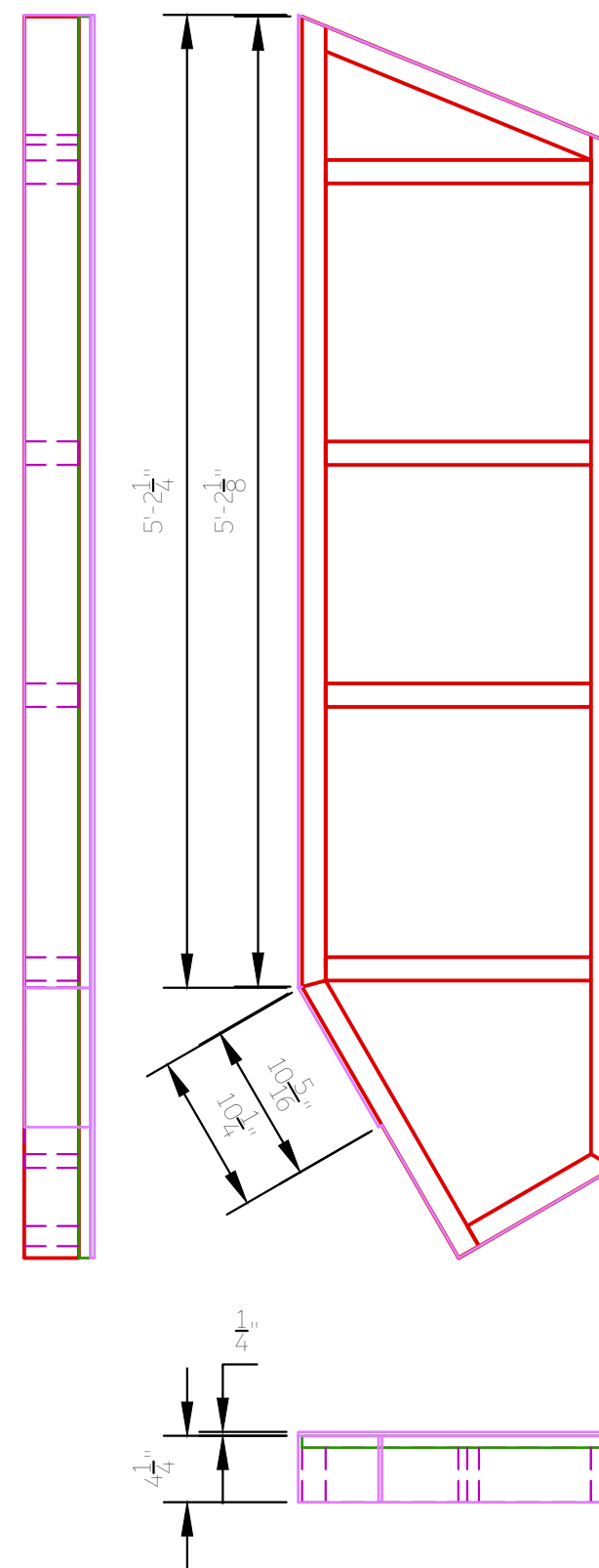
3.5 Platform 1, Section C - MDF Layout TOP, SIDE, FRONT VIEW
