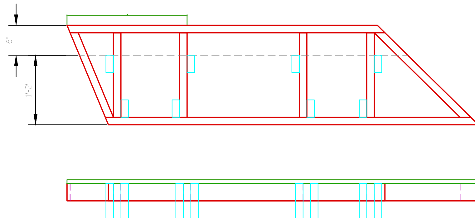
1.2 Platform 1, Section A - Leg Placement/ Inset TOP, SIDE, FRONT VIEW
