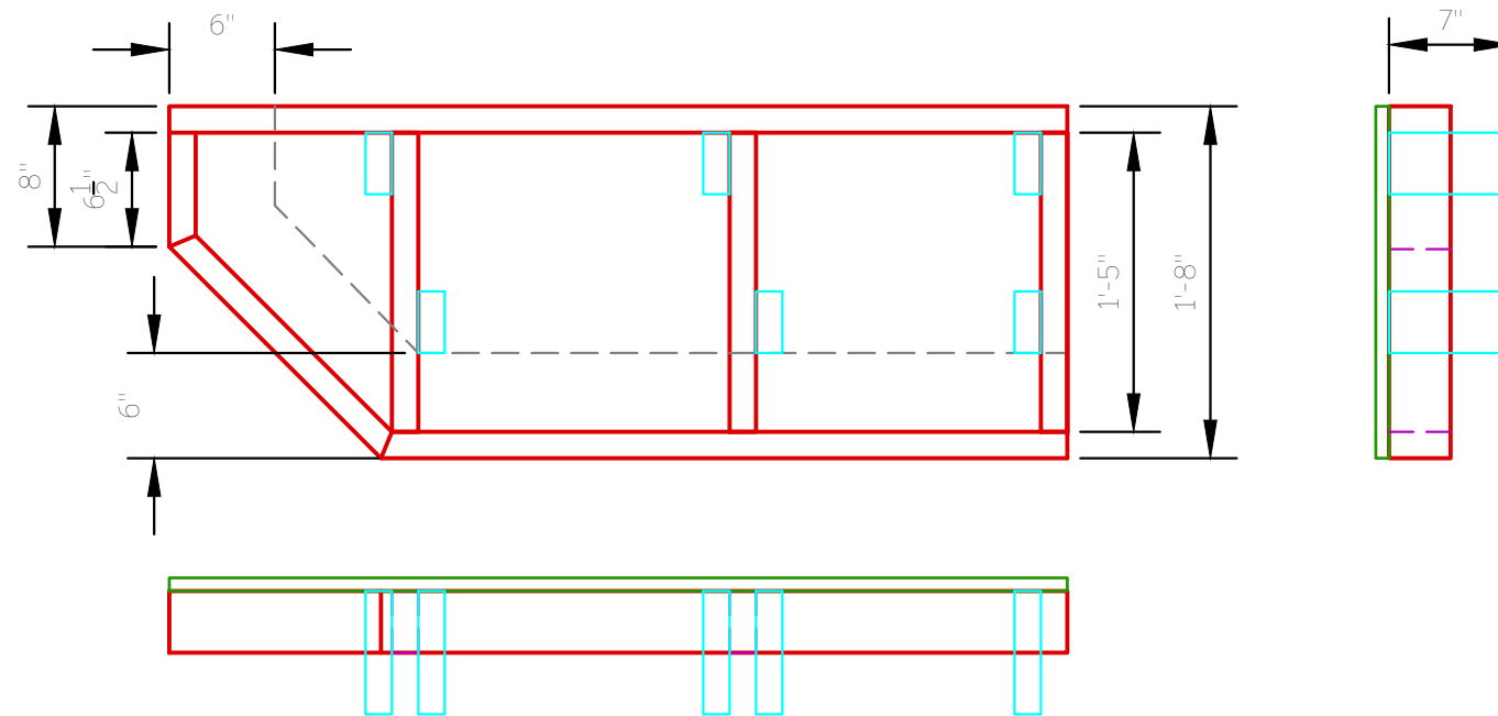
5.2 Platform 1, Sections E & F - Leg Placement/ Inset TOP, SIDE, FRONT VIEW BUILD 1 AND MIRROR; 2 TOTAL
