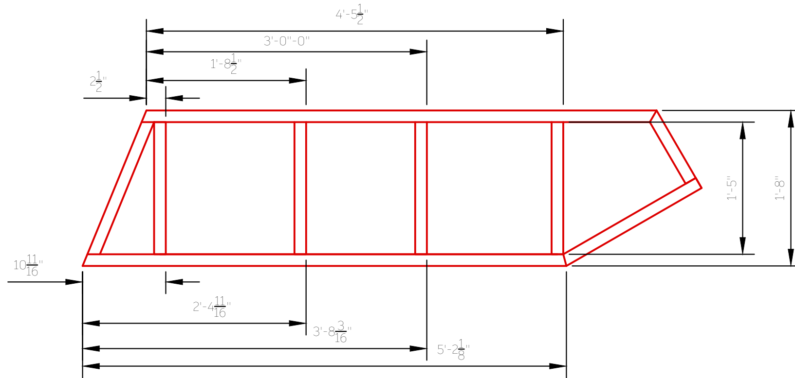
3.1 Platform 1, Section C - Toggle Placement
