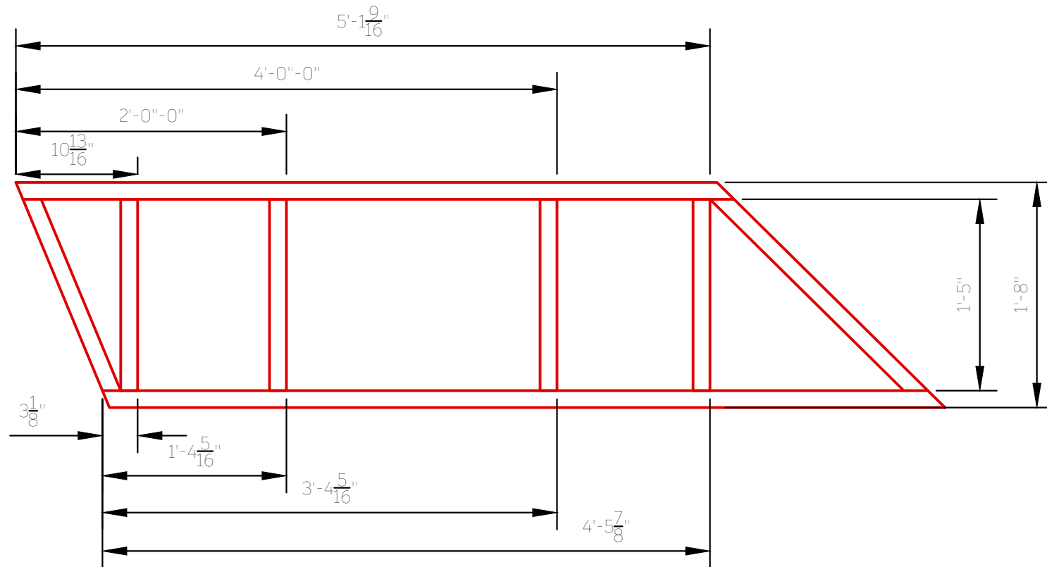
1.1 Platform 1, Section A - Toggle Placement
