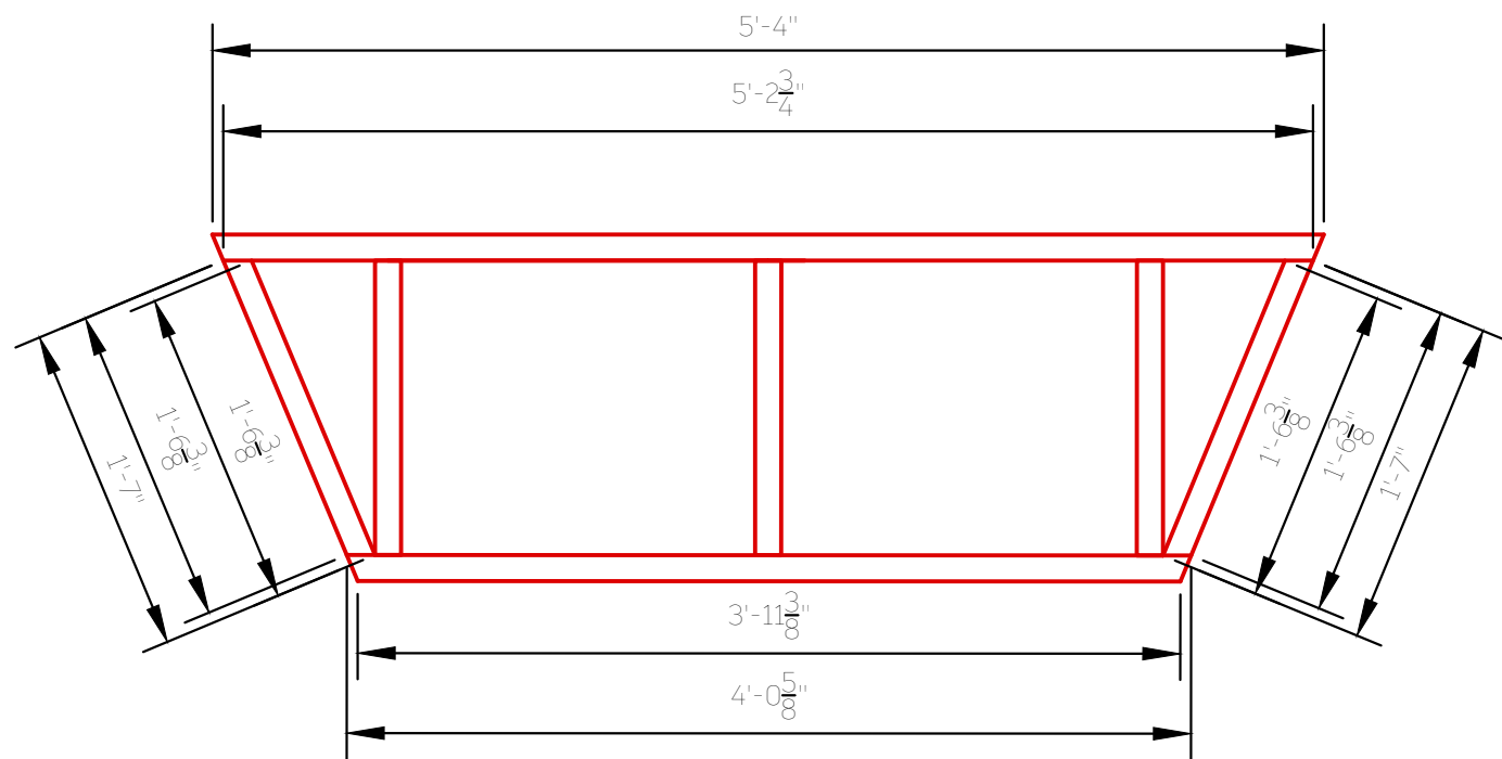
2.3 Platform 1, Section B - Angle Measurements
