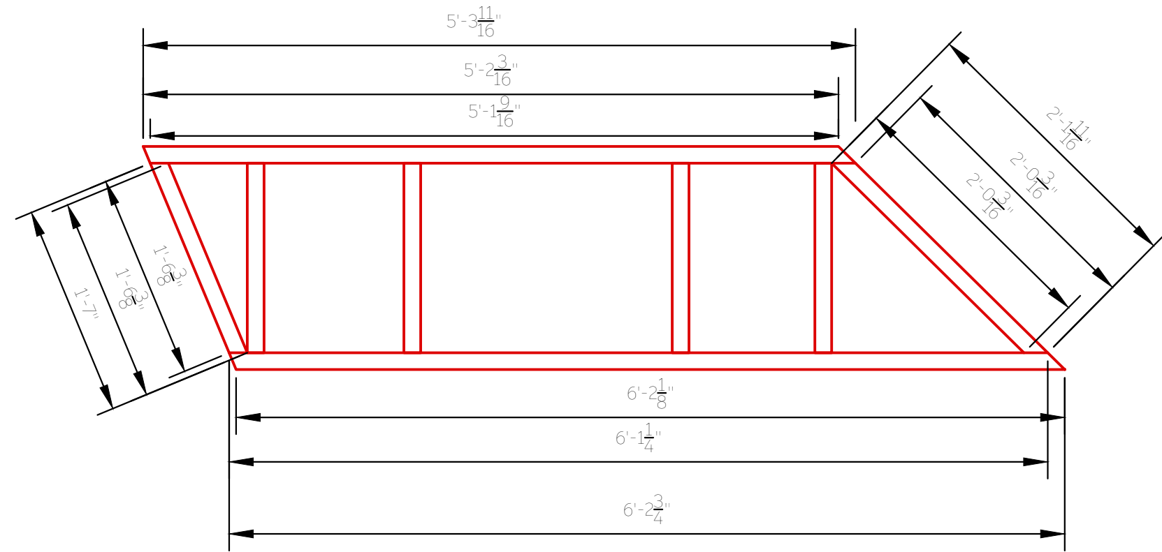
1.3 Platform 1, Section A - Angle Measurements
