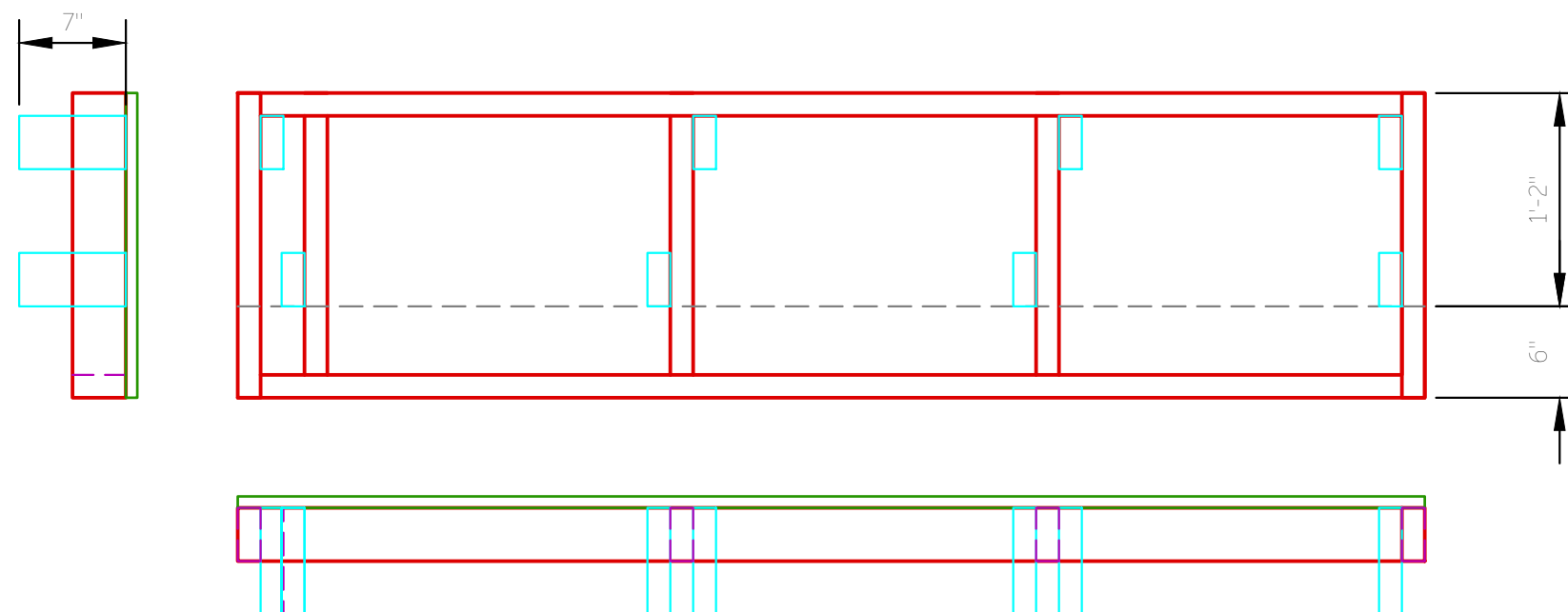
6.2 Platform 1, Section G - Leg Placement/ Inset TOP, SIDE, FRONT VIEW
