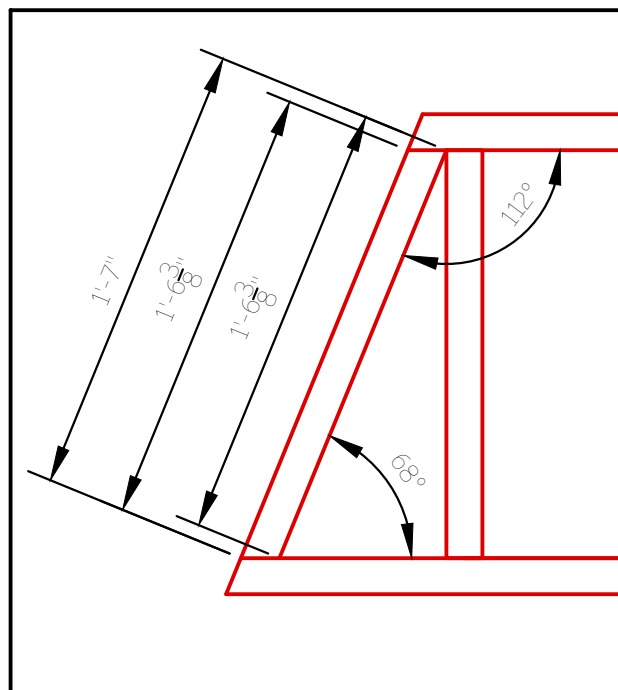
3.4 Platform 1, Section C - Angle Details
