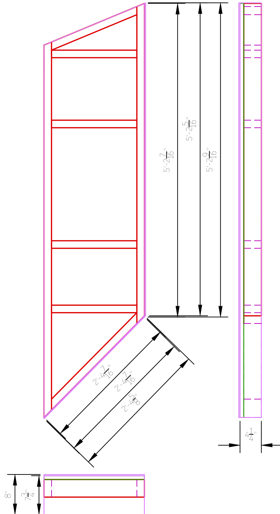
1.5 Platform 1, Section A - MDF Layout TOP, SIDE, FRONT VIEW
