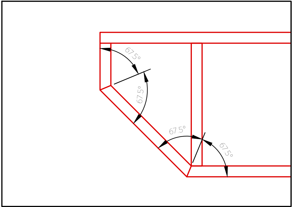
5.4 Platform 1, Sections E & F - Angle Details BUILD 1 AND MIRROR; 2 TOTAL
