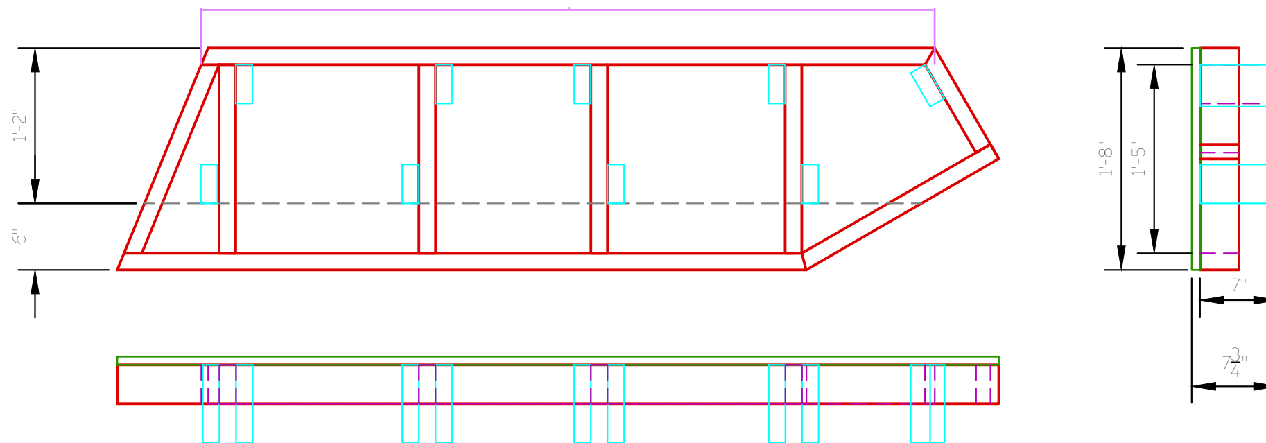
3.2 Platform 1, Section C - Leg Placement/ Inset TOP, SIDE, FRONT VIEW
