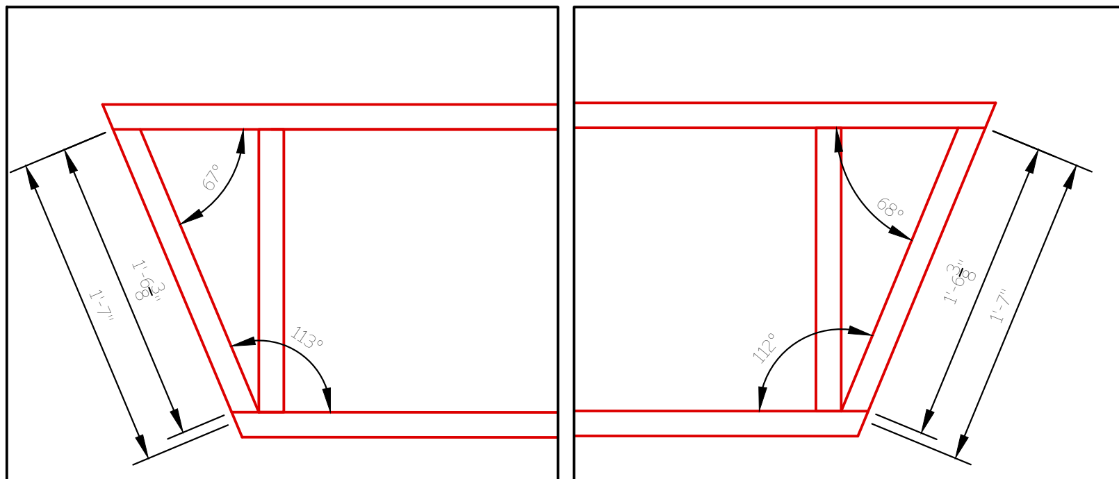
2.4 Platform 1, Section A - Angle Details
