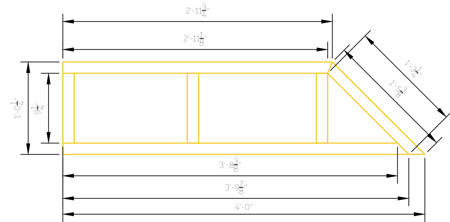
17.3 Platform 3, Section C - Angle Measurements
