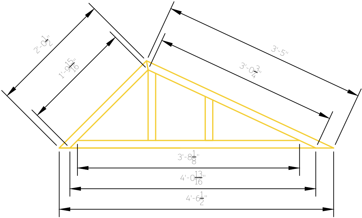
15.3 Platform 3, Section A - Angle Measurements
