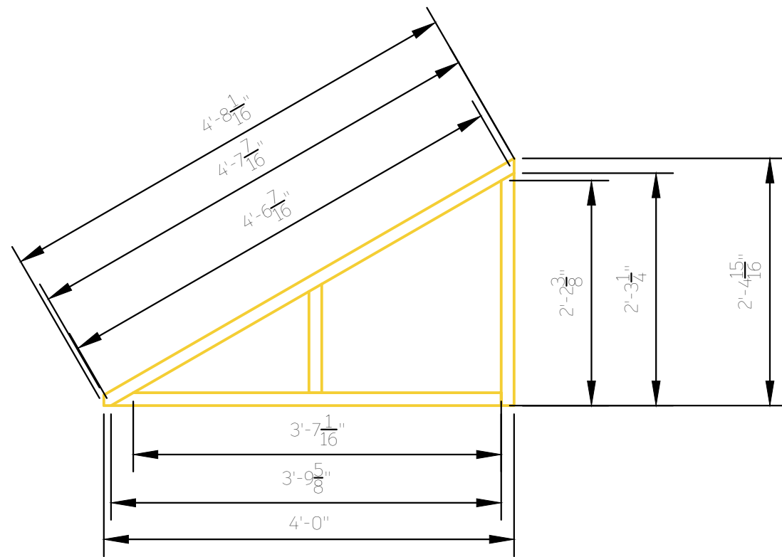
19.3 Platform 3, Section E - Angle Measurements
