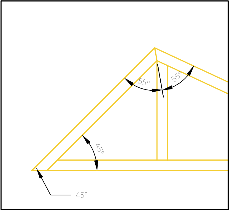
15.4 Platform 3, Section A - Angle Details
