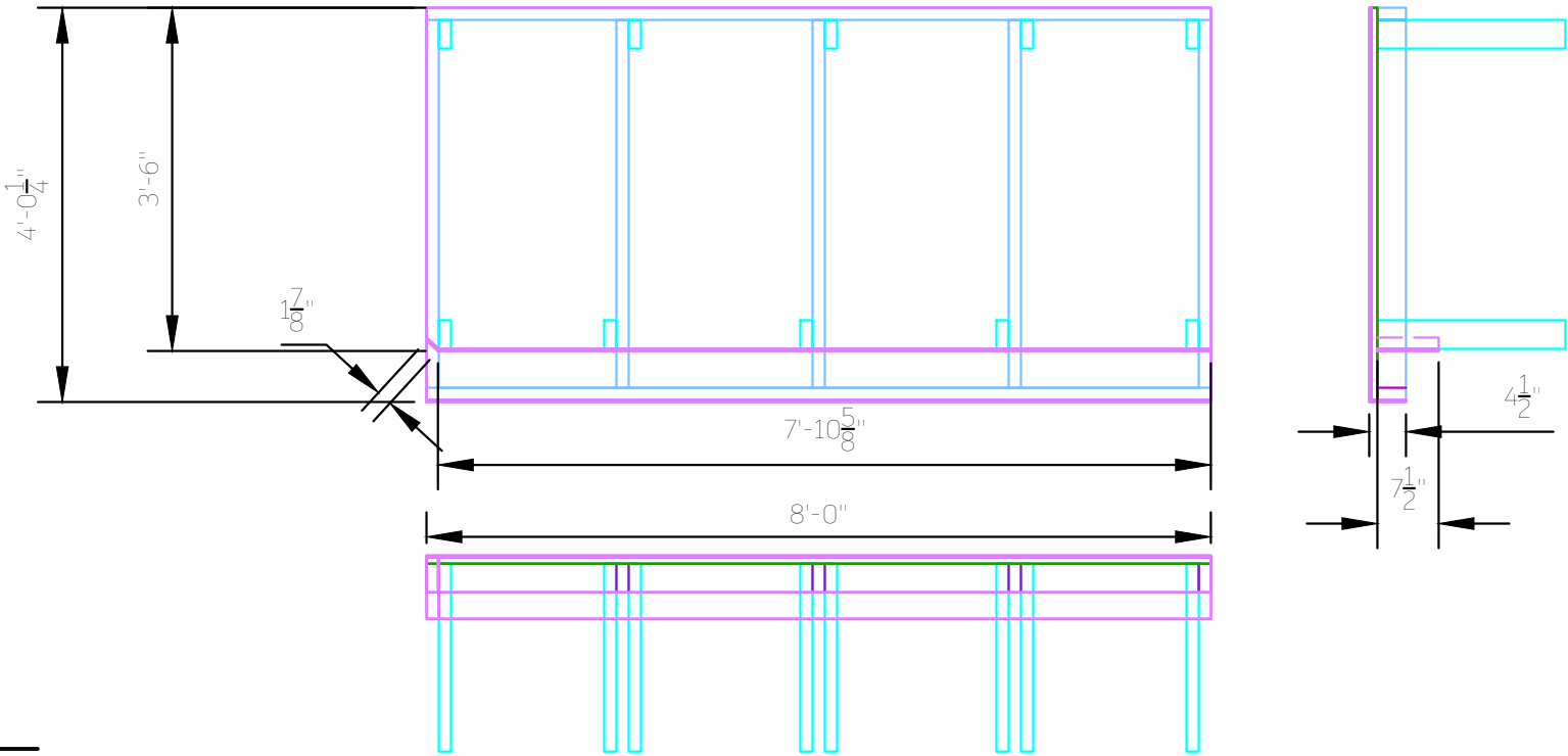
21.2 Platform 3, Section G - Stock Platform MDF TOP, SIDE, FRONT VIEW
