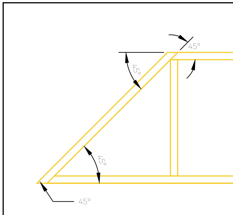
16.4 Platform 3, Section B - Angle Details
