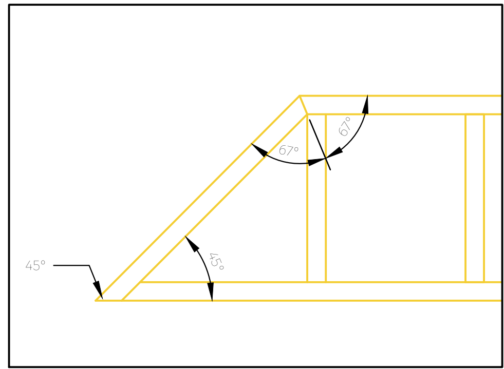
20.4 Platform 3, Section F - Angle Details
