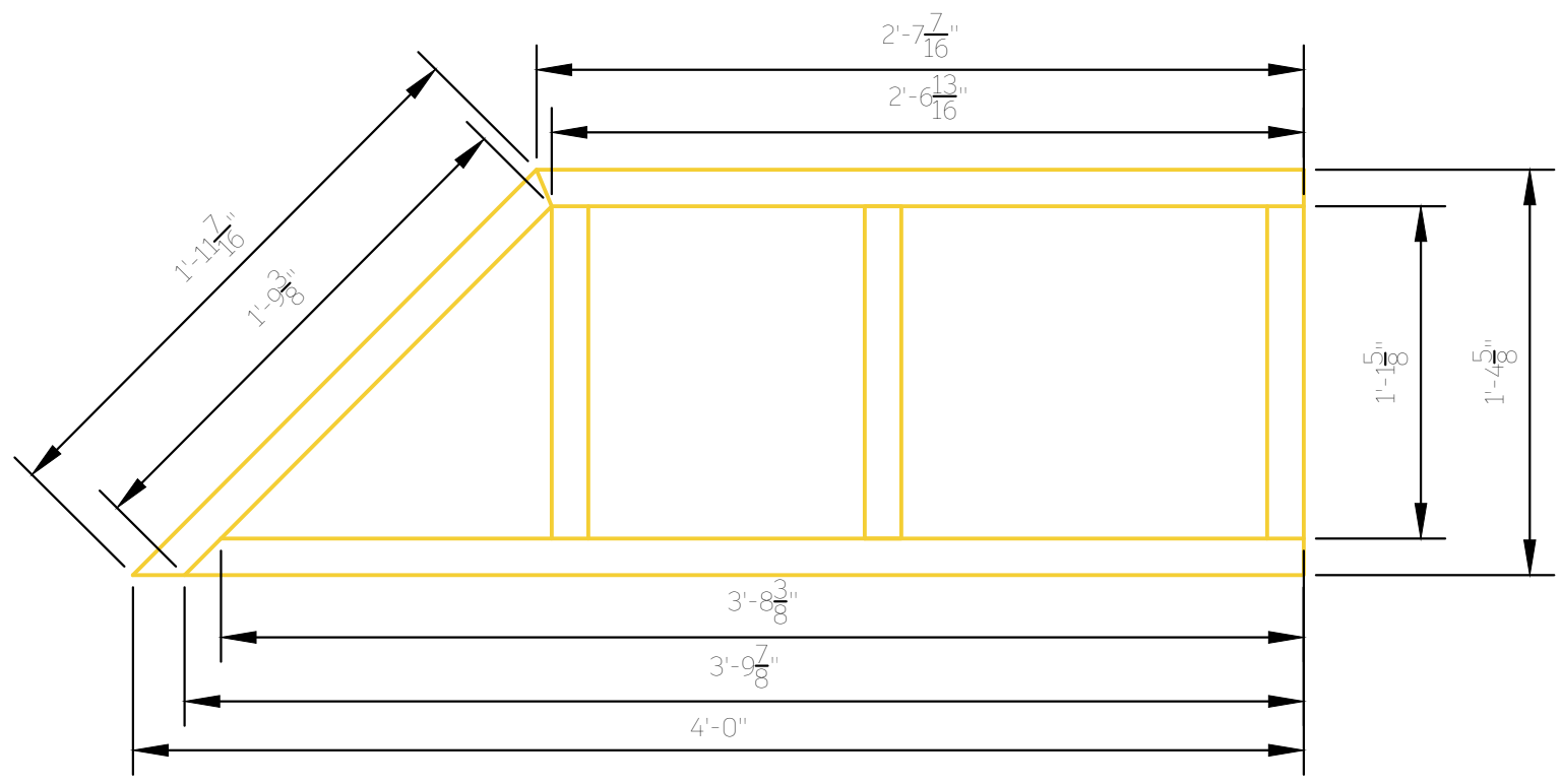
20.3 Platform 3, Section F - Angle Measurements
