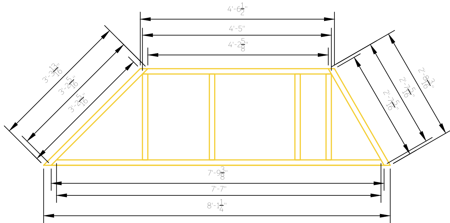
16.3 Platform 3, Section B - Angle Measurements
