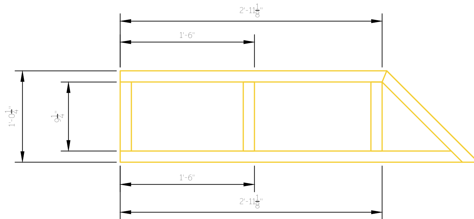
17.1 Platform 3, Section C - Toggle Placement
