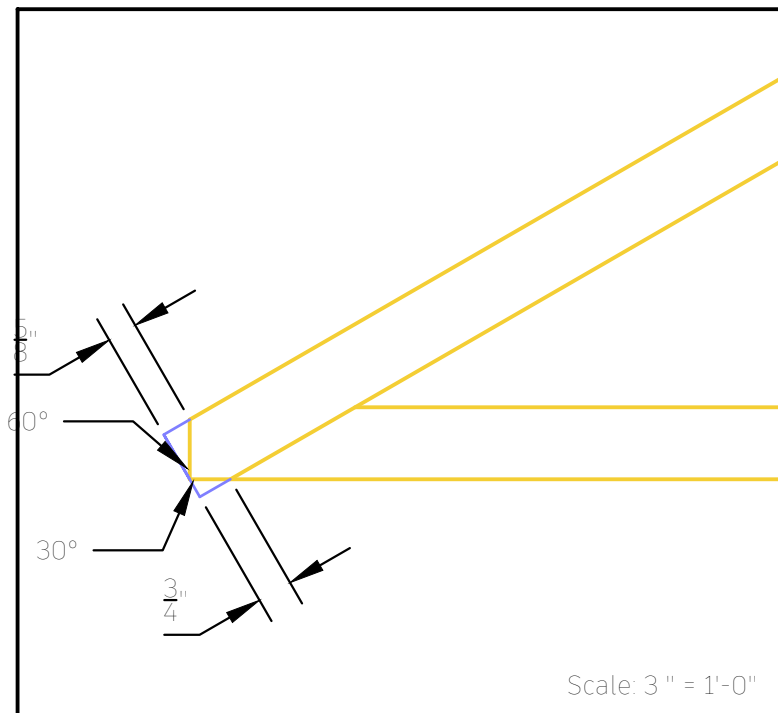
19.4 Platform 3, Section E - Angle Details
