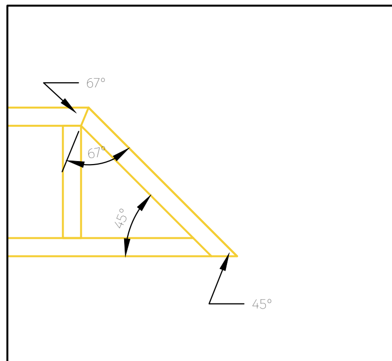
17.4 Platform 3, Section C - Angle Details
