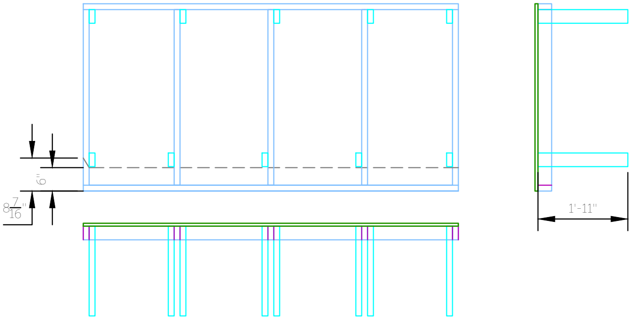
21.1 Platform 3, Section G - Stock Platform Leg Placement/ Inset TOP, SIDE, FRONT VIEW
